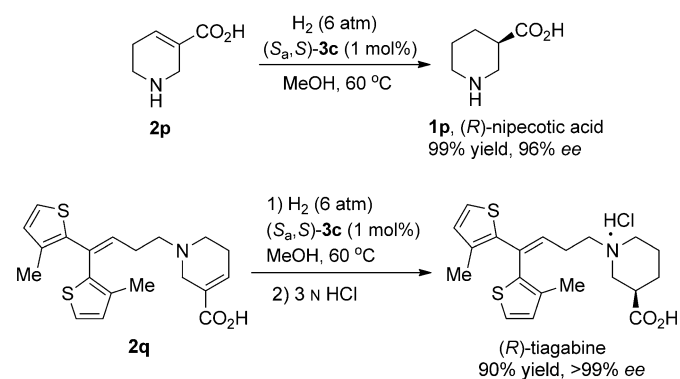
Scheme 2. The syntheses of ( R )-nipecotic acid and ( R )-tiagabine.
